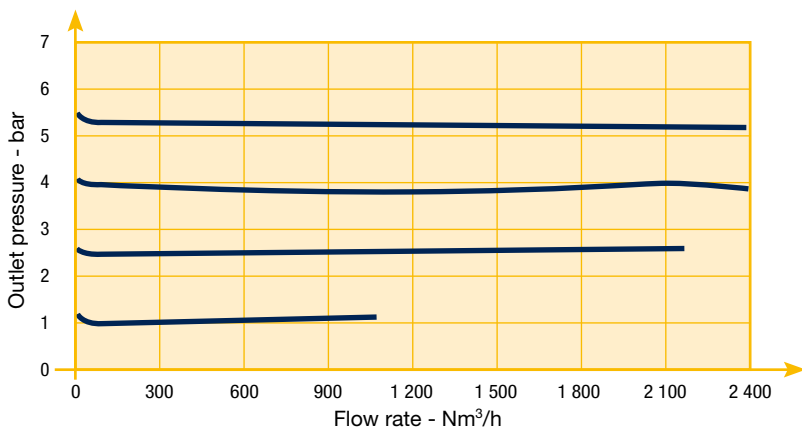
Flow Curve 2"
