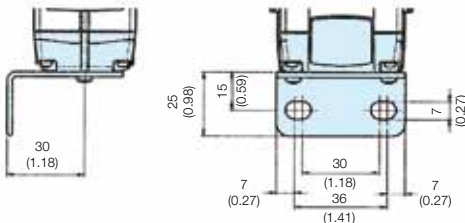
Foot Bracket
