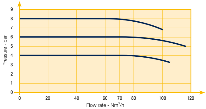
Flow Curve 1/4"
