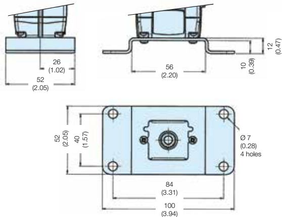
Foot Bracket
