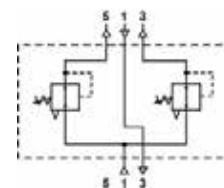
Regulation on both ports #4 & #2
