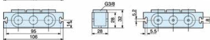
Connecting block P2N-AM513GT
